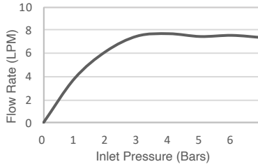
Flow Curve
