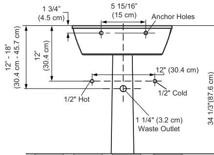
Full-Pedestal Lavatory
