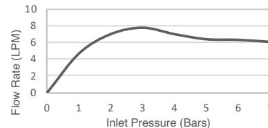
Flow Curve
