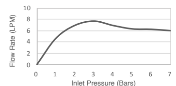
Flow Curve
