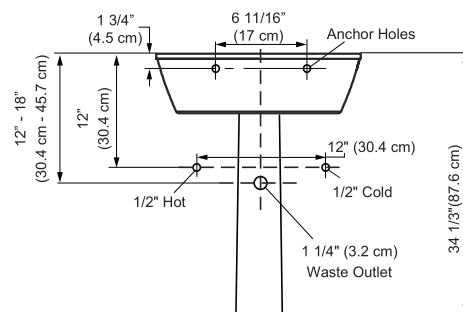
Full-Pedestal Lavatory
