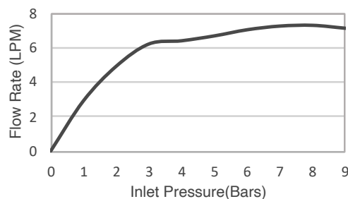
Flow Curve
