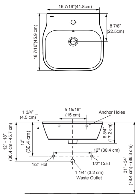
Wall Mount Lavatory Installation
