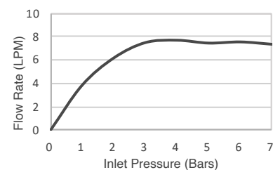
Flow Curve
