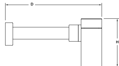
Bottle Trap Depth D, Height H mm
