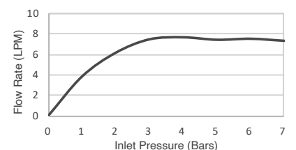
Flow Curve
