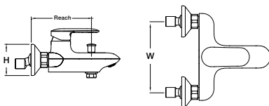
Wall-Mount exposed Bath and Shower Mixer without Hand Shower Width x Reach mm, Reach mm
