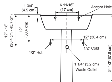
Full-Pedestal Lavatory
