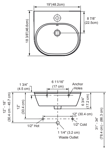
Wall Mount Lavatory Installation
