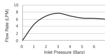
Flow Curve
