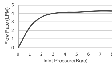
Flow Curve
