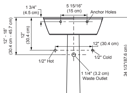
Full-Pedestal Lavatory
