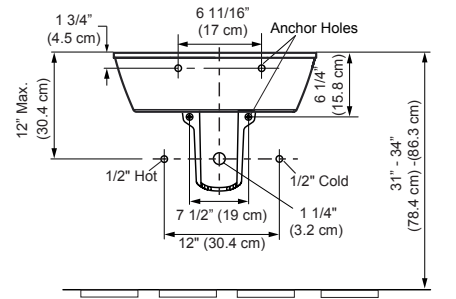
Full-Pedestal Lavatory
