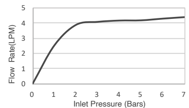
Flow Curve
