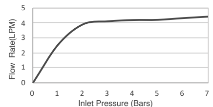
Flow Curve
