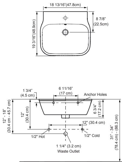
Wall Mount Lavatory Installation
