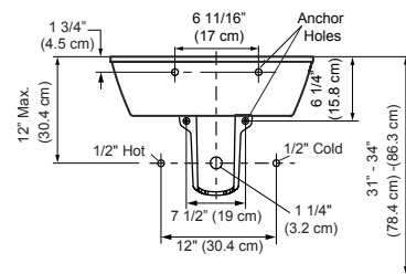
Full-Pedestal Lavatory
