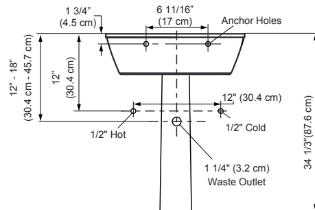
Full-Pedestal Lavatory
