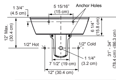
Full-Pedestal Lavatory
