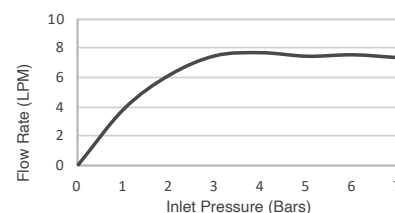
Flow Curve
