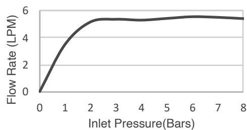
Flow graph
