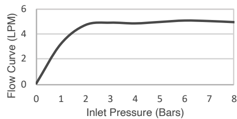
Flow Graph
