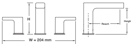
Widespread Faucet (W, Reach, Total Height H, Height till aerator mm)
