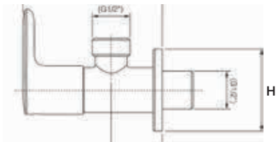
Angle Valve Height H mm
