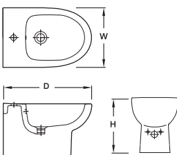
Floor-Standing Bidet (W,D,H mm)
