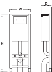
Toilets In-Wall Tank (W,D,H mm)
