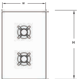
Recessed Shower Valve Trim
